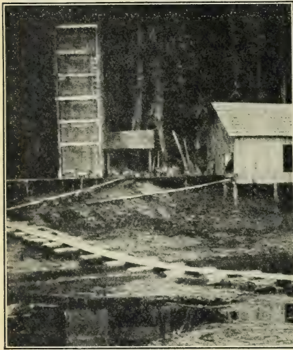
FIG. 12.—The five-tiered smokehouse illustrated will smoke and store about 5,000 salmon
